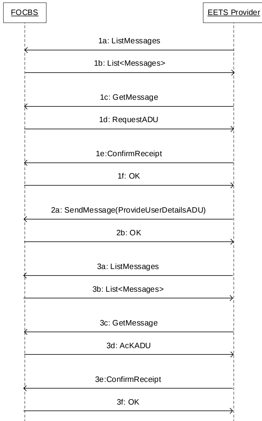
Figure 8 – FOCBS to EETS provider request message transport layer protocol
